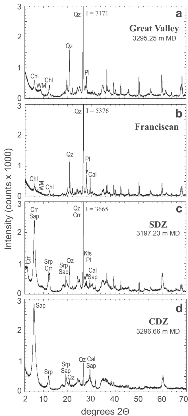
Fig. 3. X-ray diffraction (XRD) data for the SAFOD and Franciscan materials used in the friction experiments. a) Great Valley sequence; b) Franciscan mélange; c) SDZ; d) CDZ. Mineral abbreviations, after Whitney and Evans (2010) : Cal, calcite; Chl, chlorite; Crr, corrensite; Kfs, K-feldspar; WM, white mica (illite and illite-smectite in a, phengite in b); Qz, quartz; Pl, plagioclase. I = intensity of quartz (101) peak at 26.65° 2θ. Mineral identifications were verified using scanning electron microscope and electron microprobe techniques.
