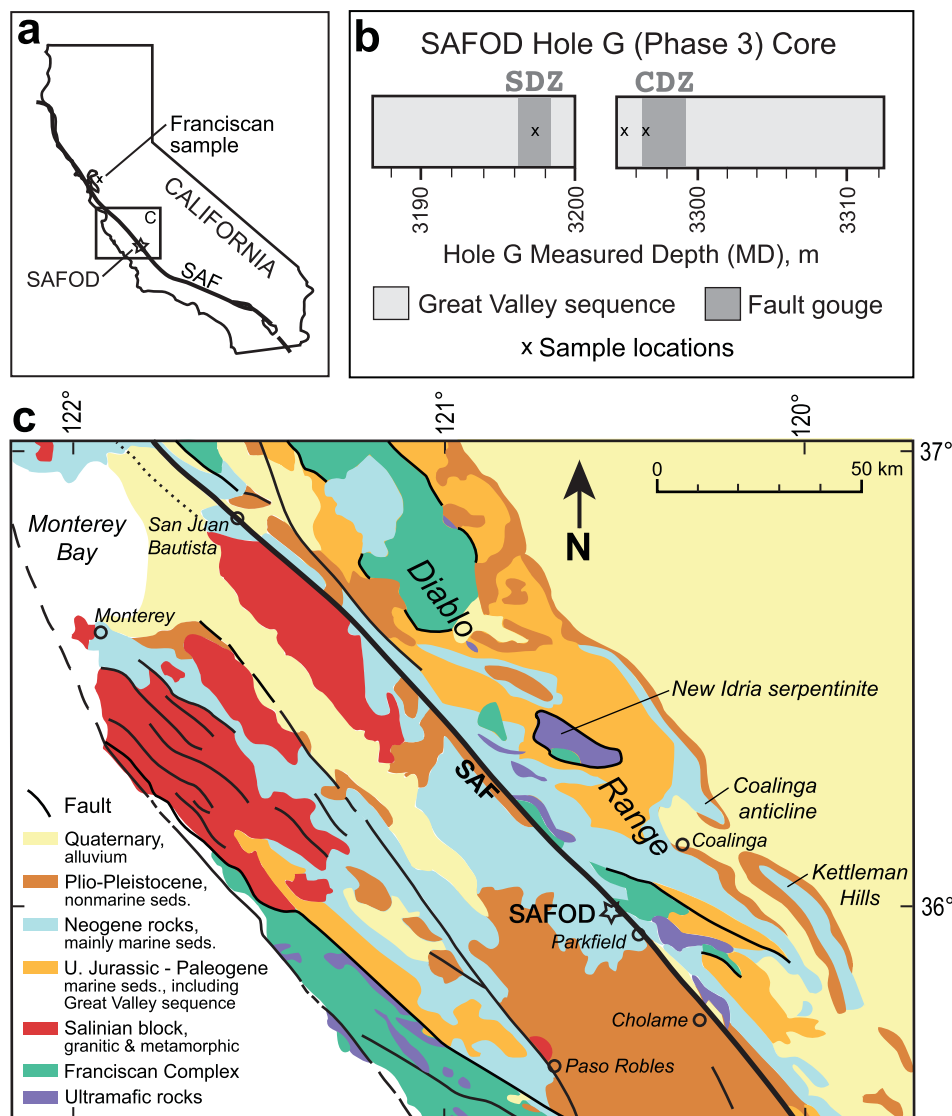
Fig. 1. Sample locations and regional geology of the creeping section of the San Andreas Fault (SAF). a ) General sample locations. The Franciscan sample was collected in the San Francisco Bay area; the other three are from the SAFOD drillhole. The box outlines the area of the geologic map in c ). b ) Fault gouge and Great Valley sample positions in the SAFOD Hole G core. c ) Simplified geologic and fault map of a portion of central California, modified from Jennings et al. (1977) with additional information from Page et al. (1998) and Titus et al. (2011). The SAFOD drillhole initiated in granitic rocks southwest of the SAF and terminated in the Great Valley sequence on the northeast side.
