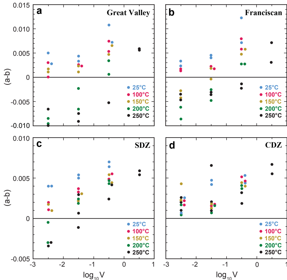
Fig. 9. Summary of velocity data, (a-b) , in the temperature range 25°–250 °C for a) Great Valley, b) Franciscan, c) SDZ, and d) CDZ samples. Data are plotted at the midpoints of velocity steps; some data points are shifted slightly to improve visibility. All of the data and error estimates are presented in Supplementary Tables 3–6 .
