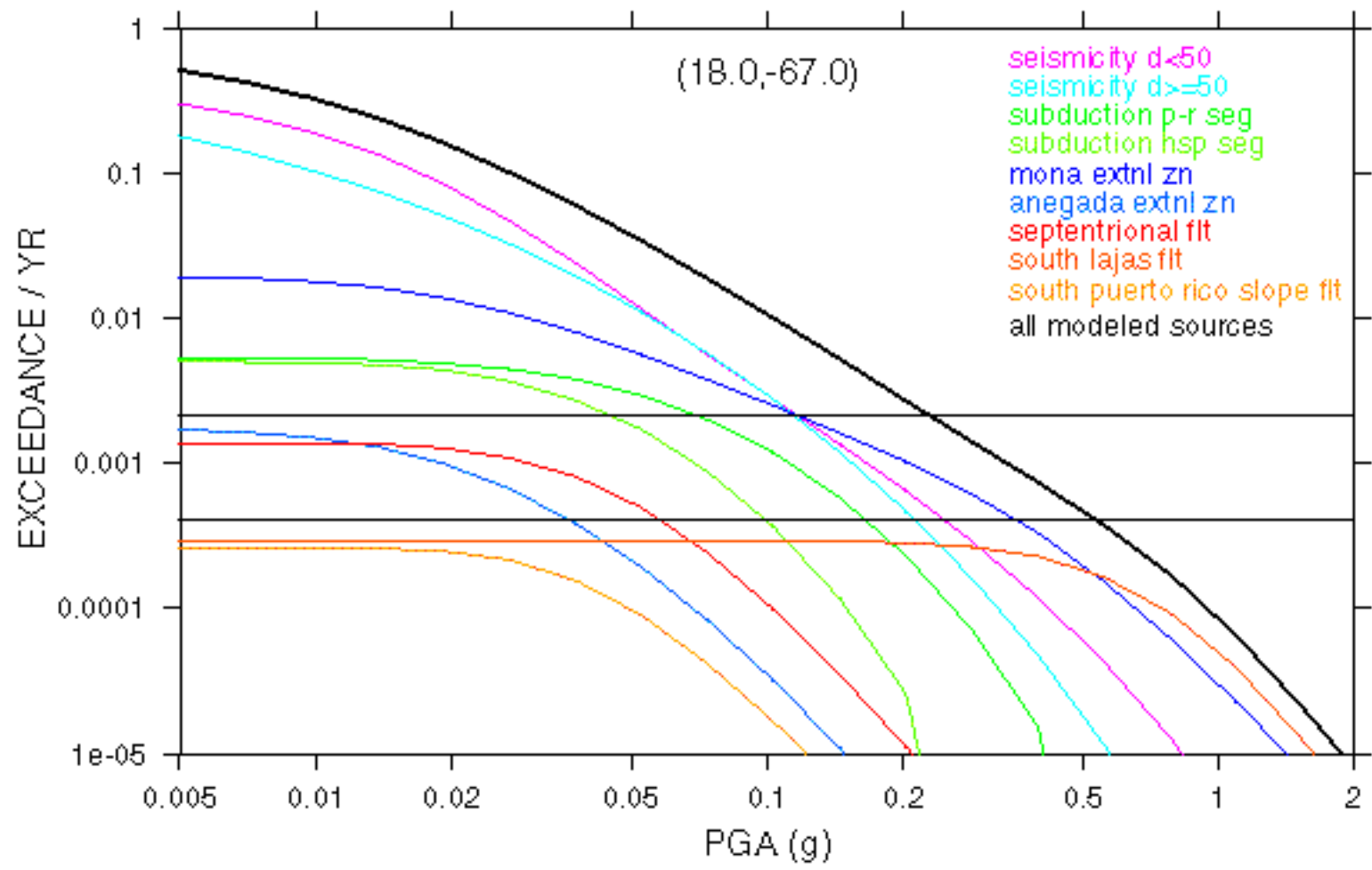
Fig.13f: PGA hazard curves for southwest Puerto Rico (18.0,-67.0).
