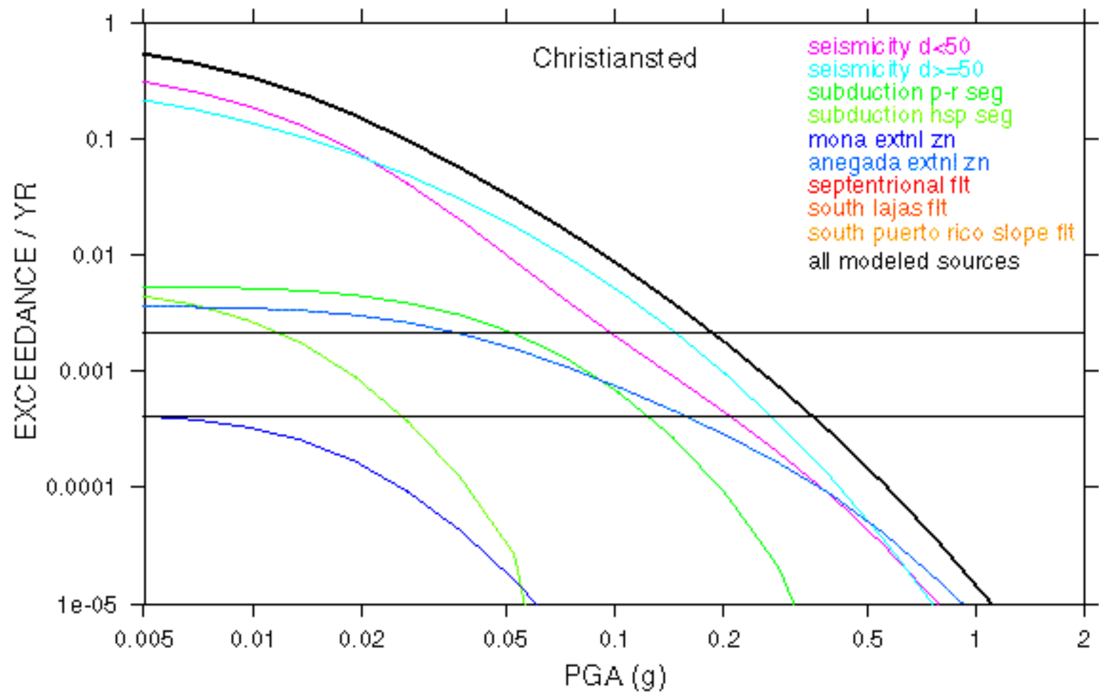
Fig.13e: PGA hazard curves for Christiansted.
