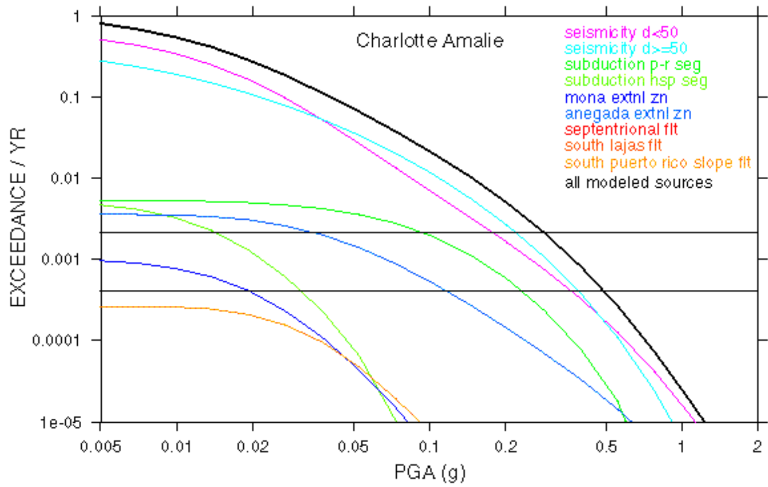
Fig.13d: PGA hazard curves for Charlotte Amalie.
