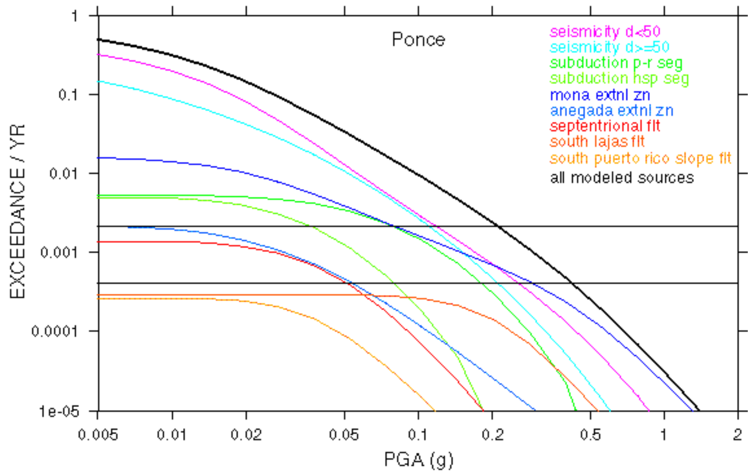
Fig.13c: PGA hazard curves for Ponce.
