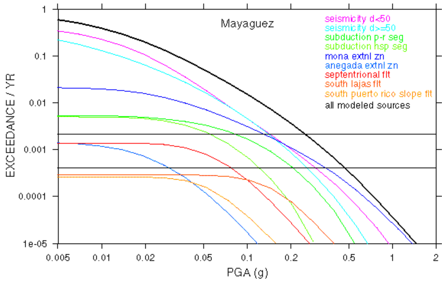
Fig.13b: PGA hazard curves for Mayaguez.
