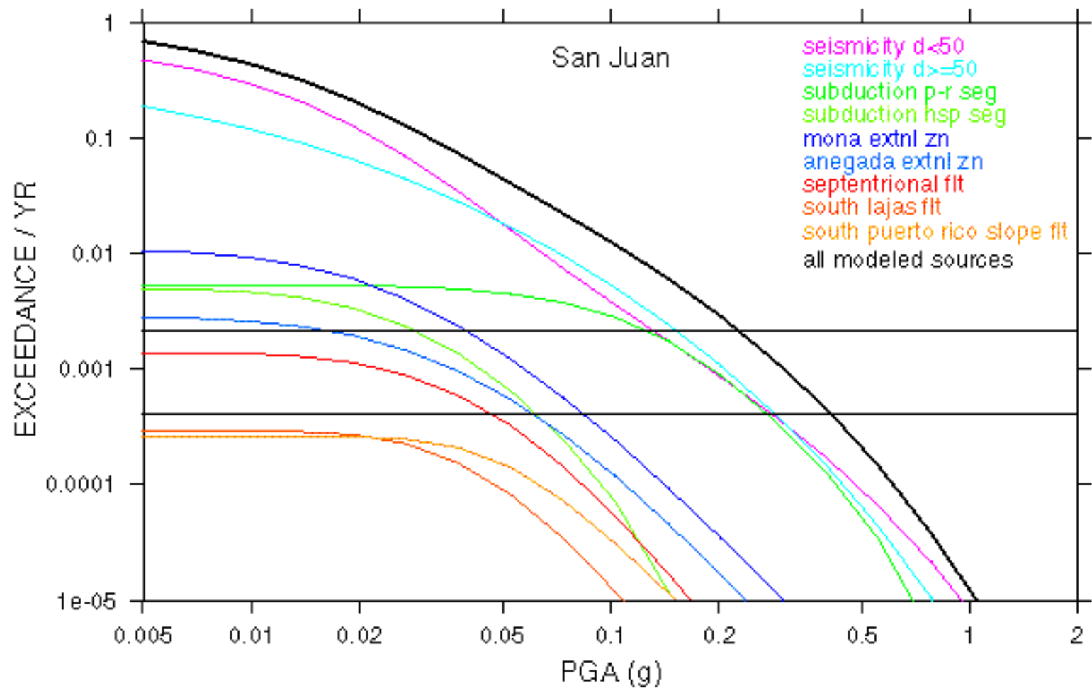
Fig.13a: PGA hazard curves for San Juan.
