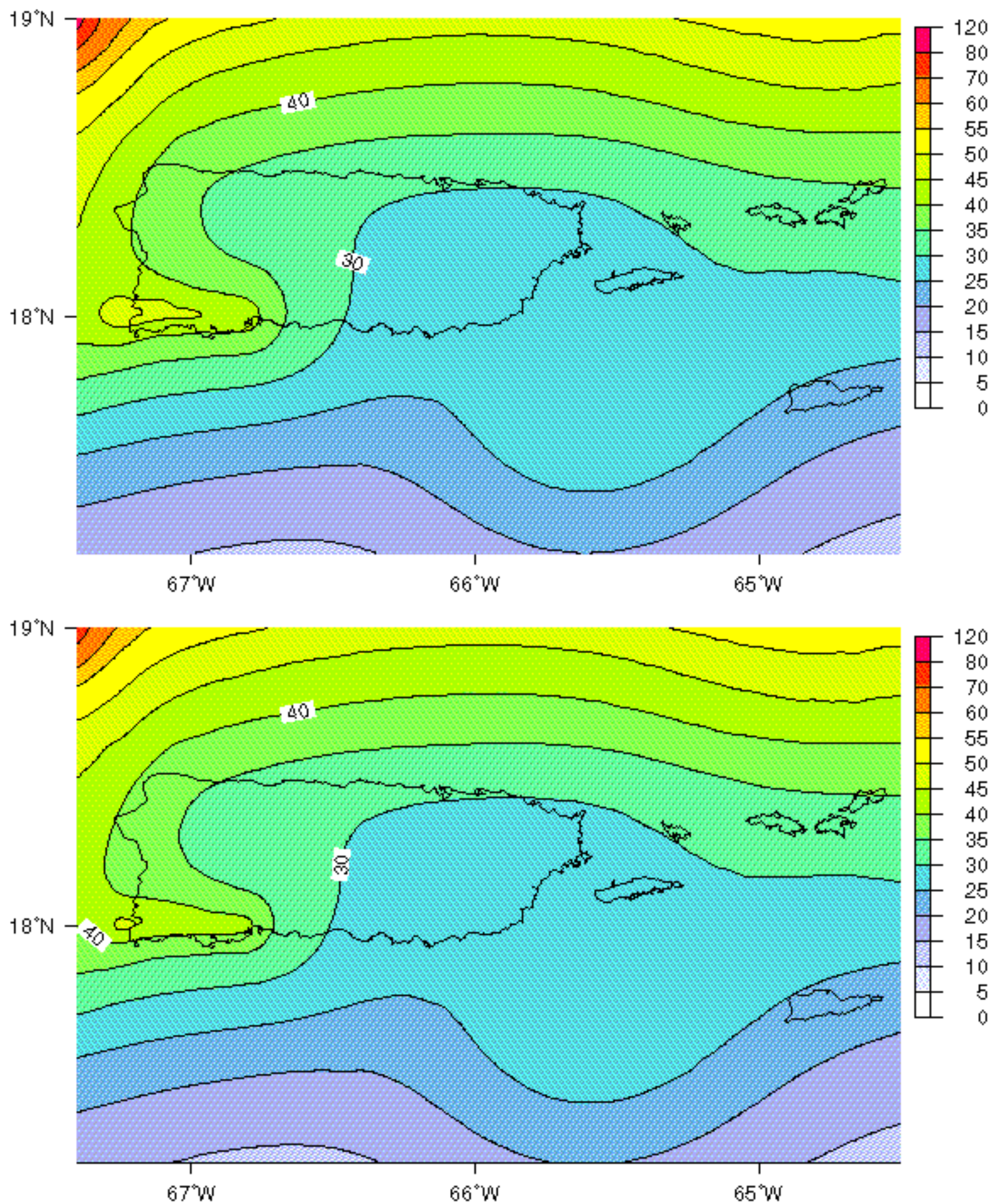
Fig.12: 1.0-second spectral acceleration (%g) with 2% probability of exceedance in 50 years from all modeled sources. Compare 50% (top) and 10% (bottom) weights for Motazedian & Atkinson (2003) attenuation.
