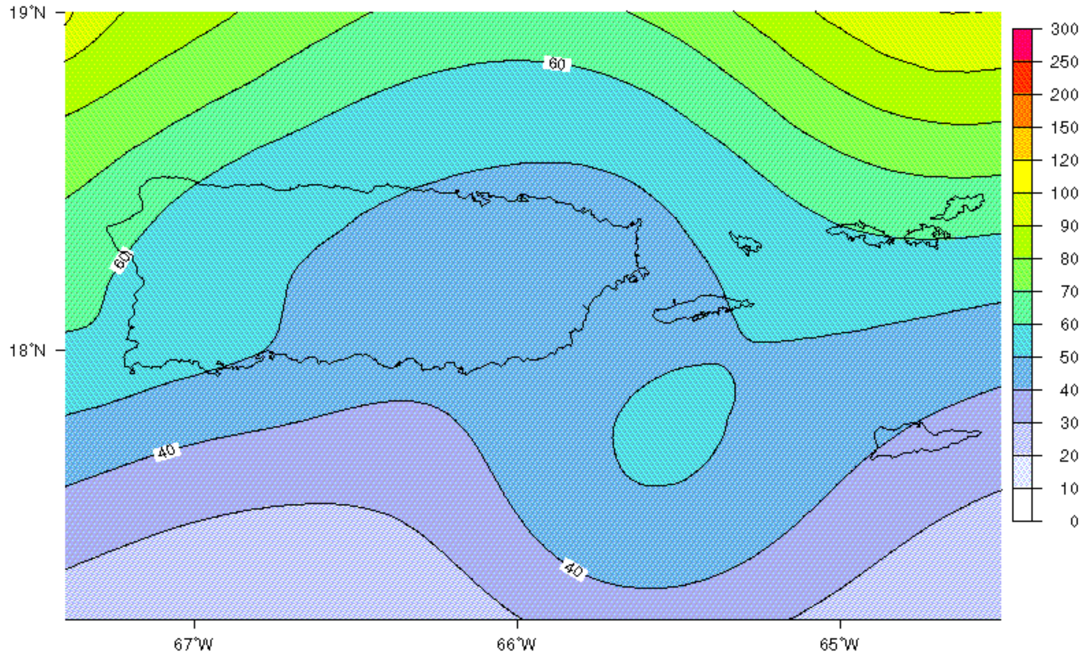
Fig.9: 0.2-sec spectral acceleration (%g) with 10% probability of exceedance in 50 years from all modeled sources.
