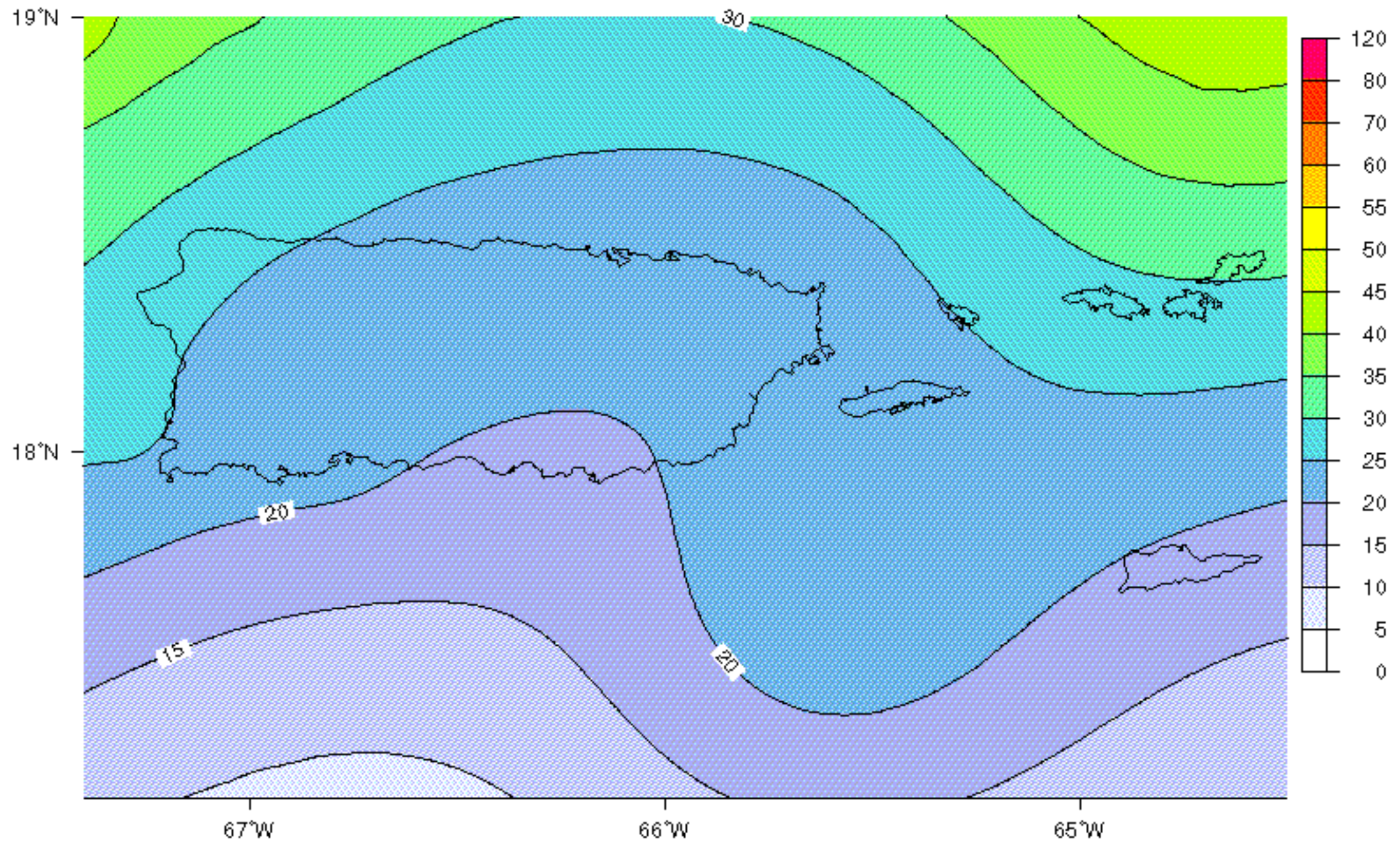
Fig.7: PGA (%g) with 10% probability of exceedance in 50 years from all modeled sources.
