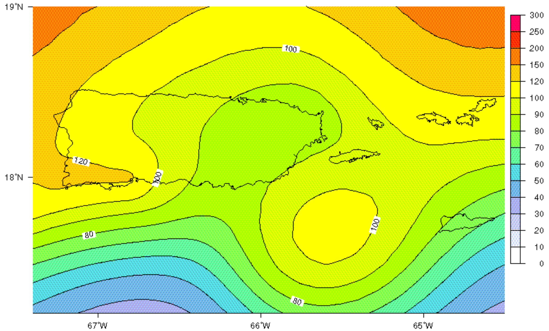
Fig.6: 0.2-sec spectral acceleration (%g) with 2% probability of exceedance in 50 years from all modeled sources.
