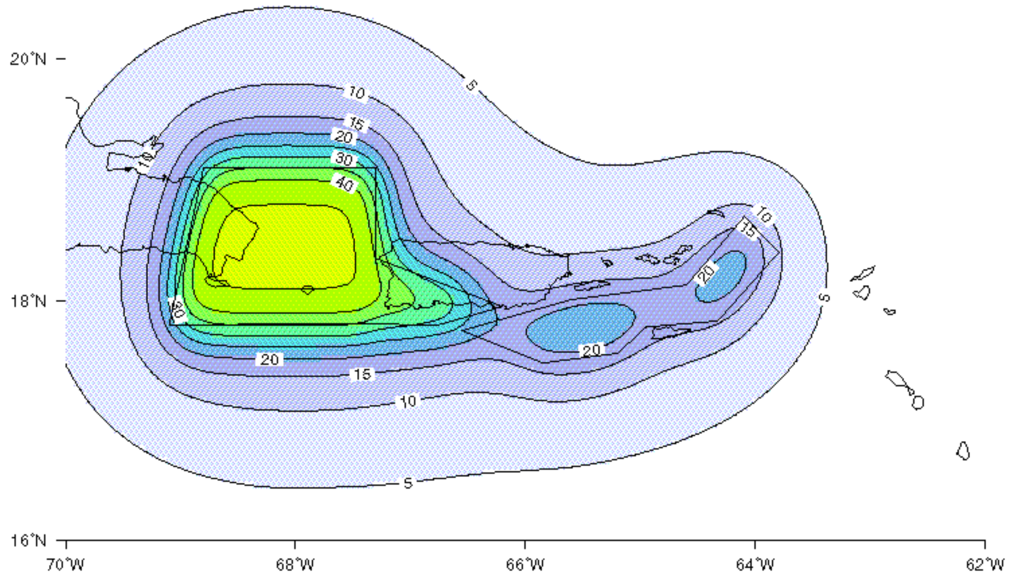
Fig.3e: PGA (%g) with 2% probability of exceedance in 50 years from Anegada and Mona extensional zones.
