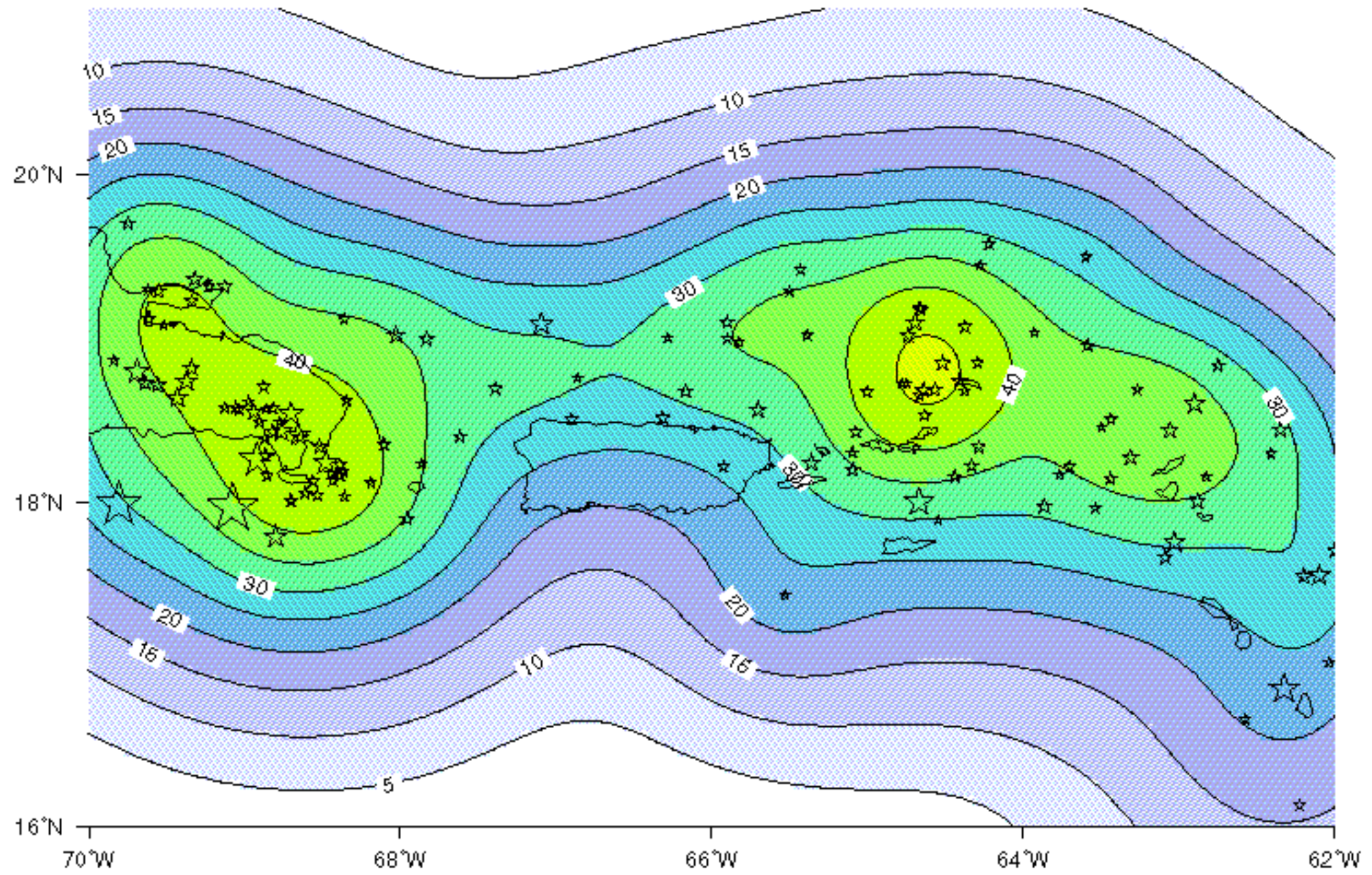
Fig.3b: PGA (%g) with 2% probability of exceedance in 50 years from deep seismicity ( d \geq 50\text{km} ).
