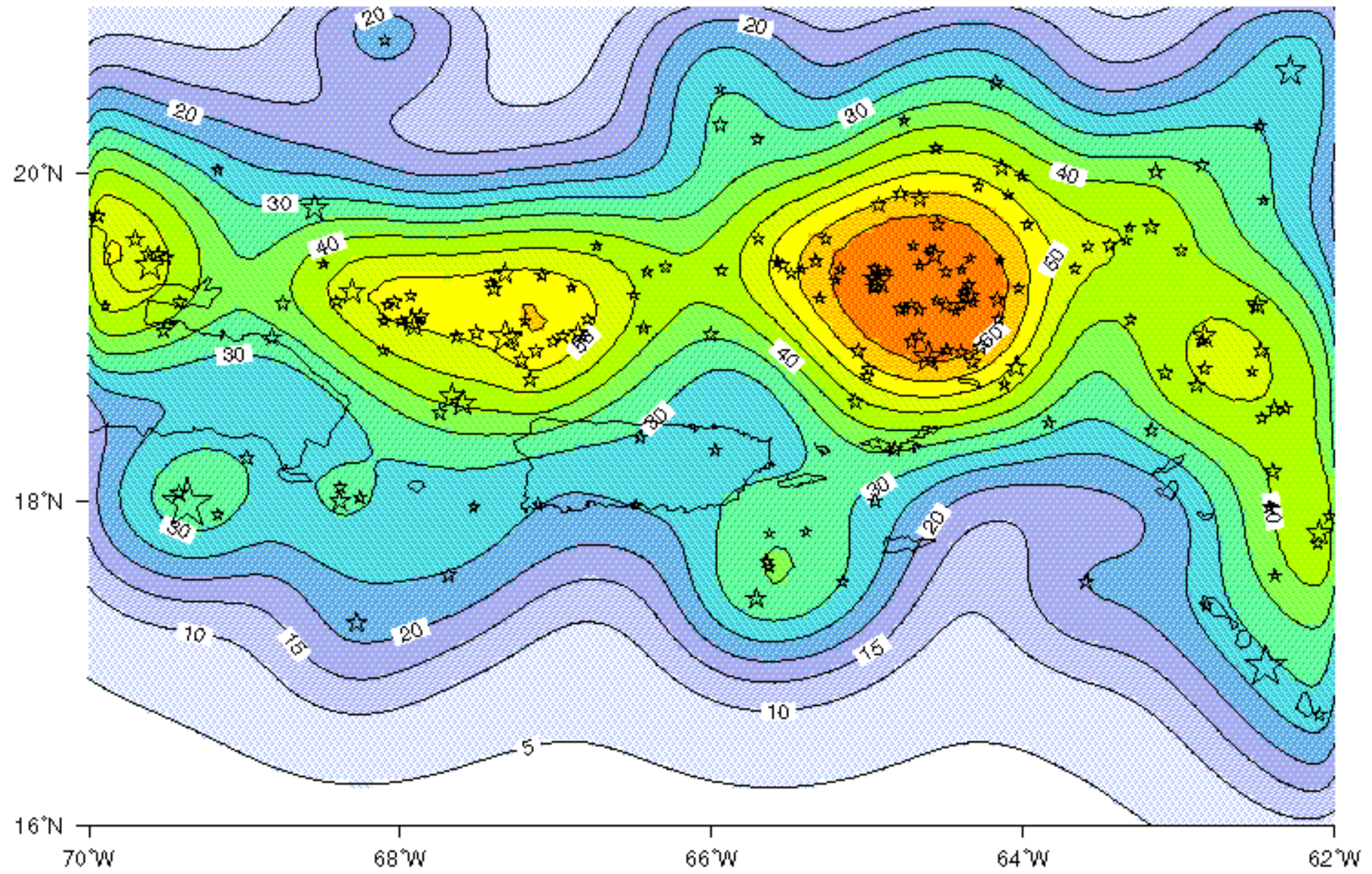
Fig.3a: PGA (%g) with 2% probability of exceedance in 50 years from shallow seismicity ( d < 50\text{km} ).
