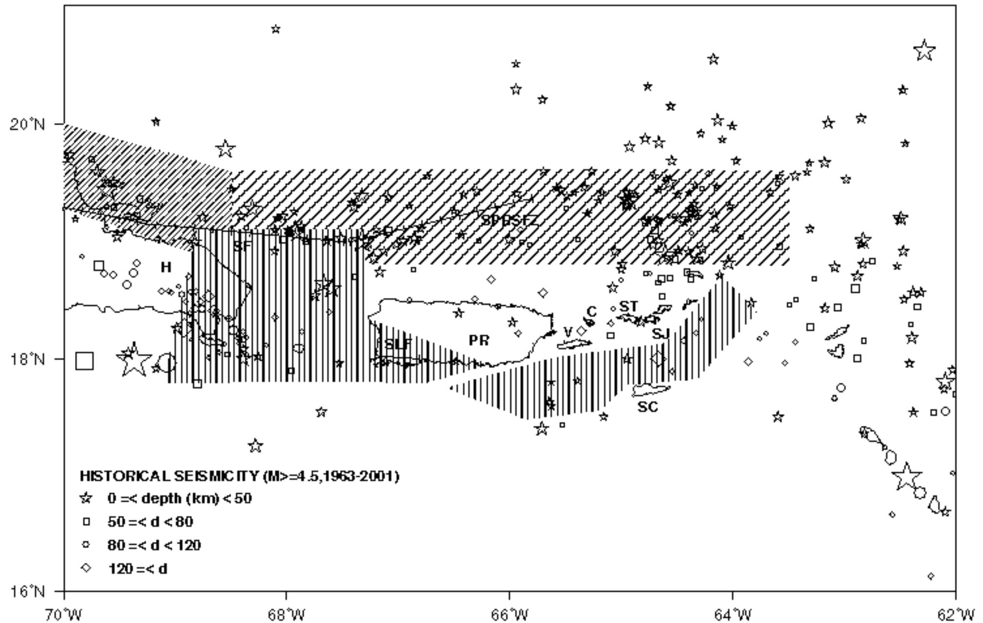
Fig.2: Map showing modeled seismic hazard sources. Diagonal pattern= subduction segments (sparse= Puerto Rico seg., dense= Hispaniola seg.). Vertical pattern= Mona and Anegada extensional zones. SF= Septentrional fault. SPRSFZ= South Puerto Rico Slope fault zone. SLF= South Lajas fault. Abbreviations: H=Hispaniola, PR= Puerto Rico, V= Vieques, C= Culebra, SC= St. Croix, ST= St. Thomas, SJ= St. John.
