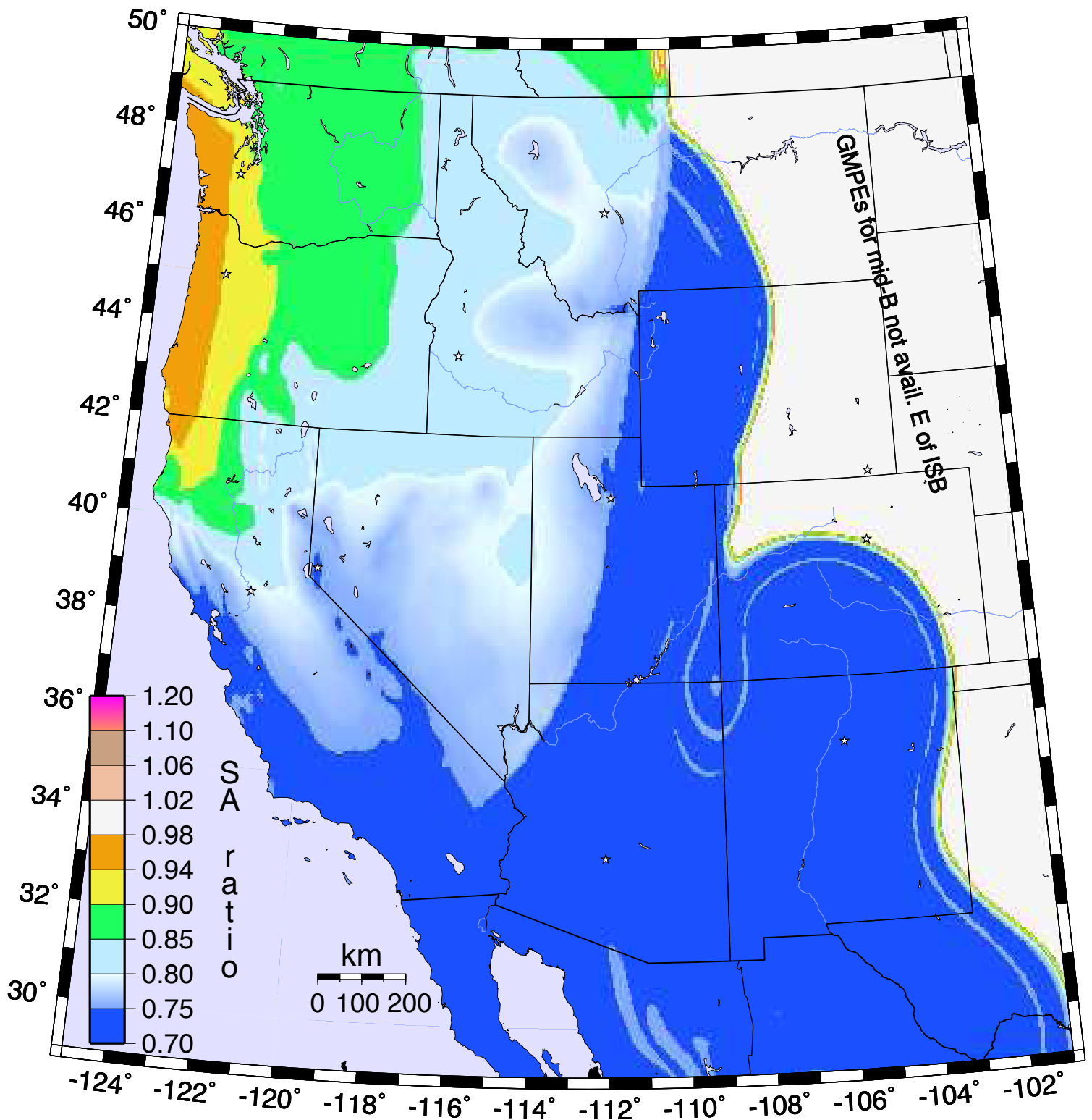
Ratio 0.5-Hz SA, 2% PE in 50y, for Site Classes B/BC.
