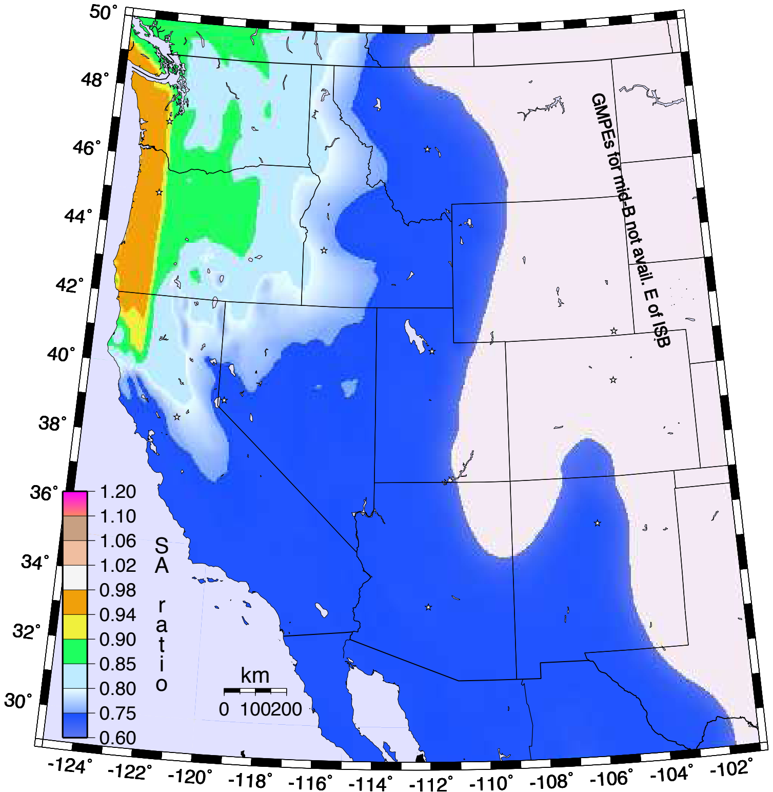
Ratio 1-Hz SA, 2% PE in 50y, for Site Classes B/BC.
