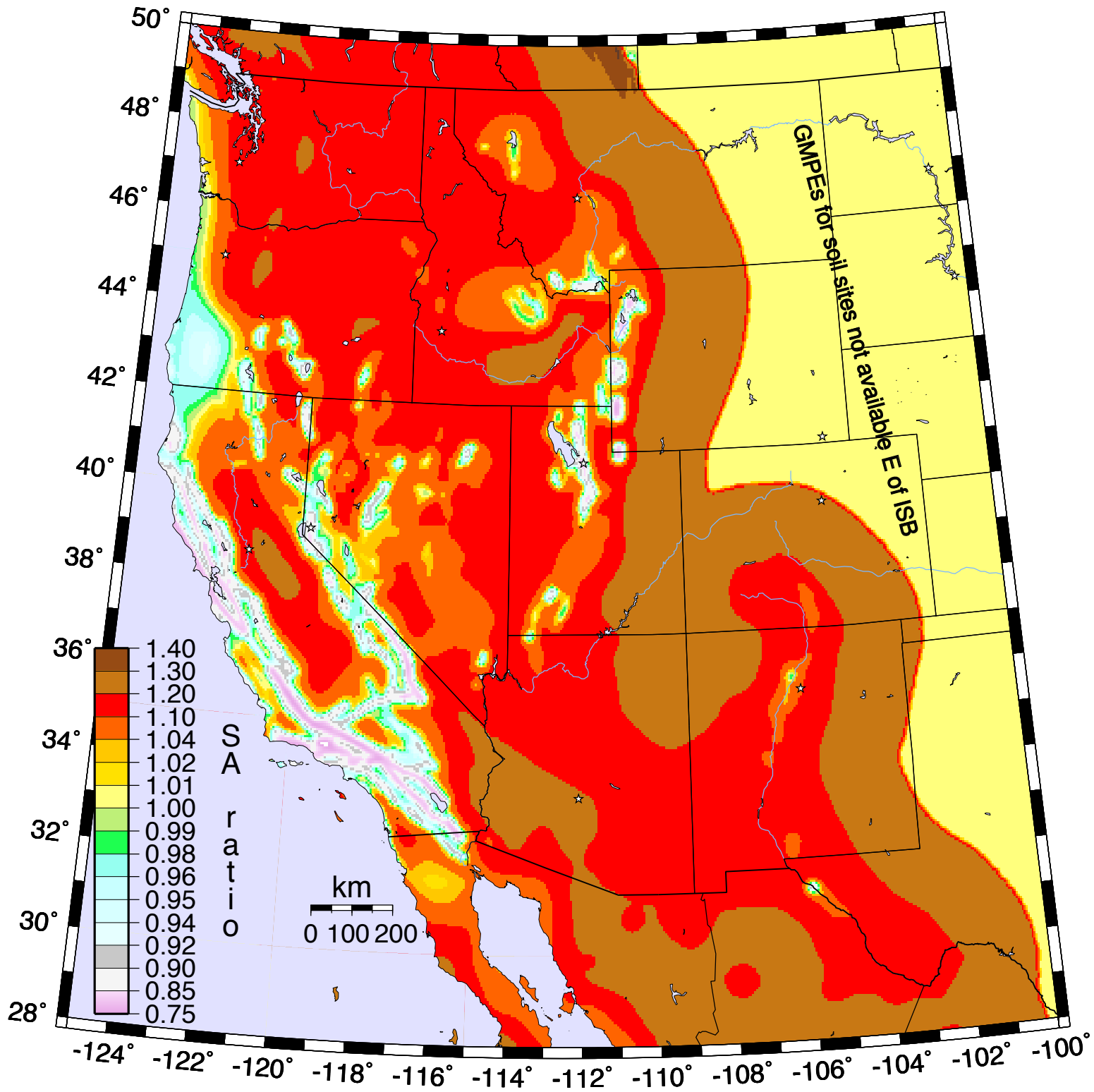
Ratio 3.33-Hz SA, 2% in 50y, for Site Class DE/D (180, 259 m/s)
