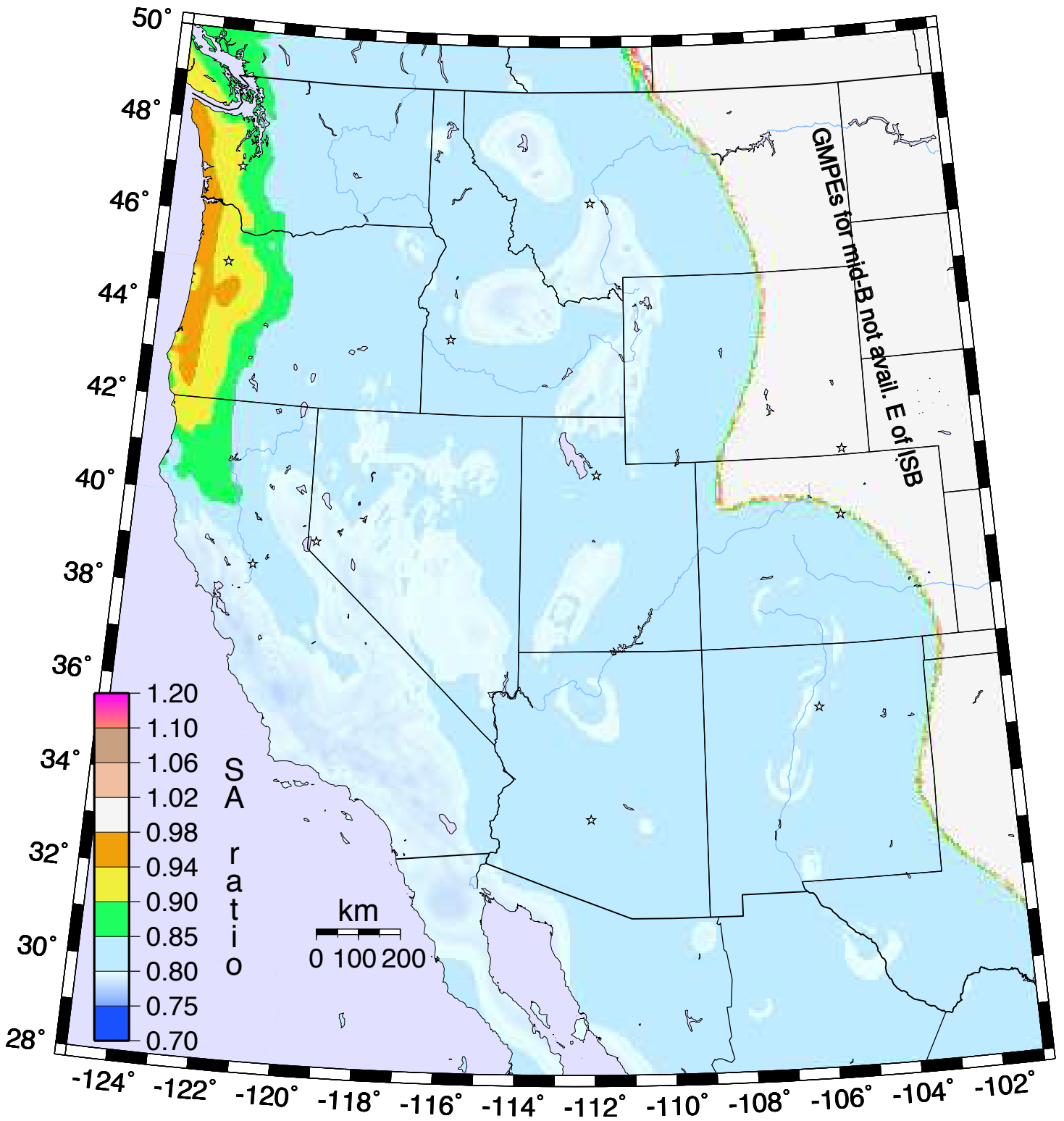
Ratio 3.33-Hz SA, 2% in 50y, for Site Class B/BC.
