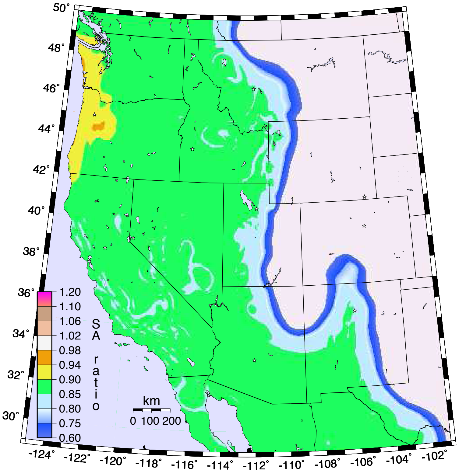
Ratio 5-Hz SA, 2% in 50y, for Site Class B/BC.
