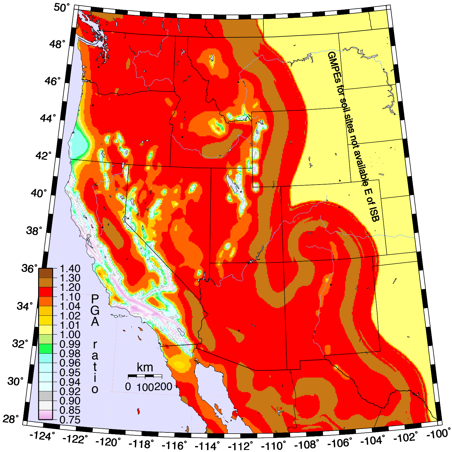
Ratio PGA, 2% in 50y, for Site Class DE/D (180, 259 m/s).
