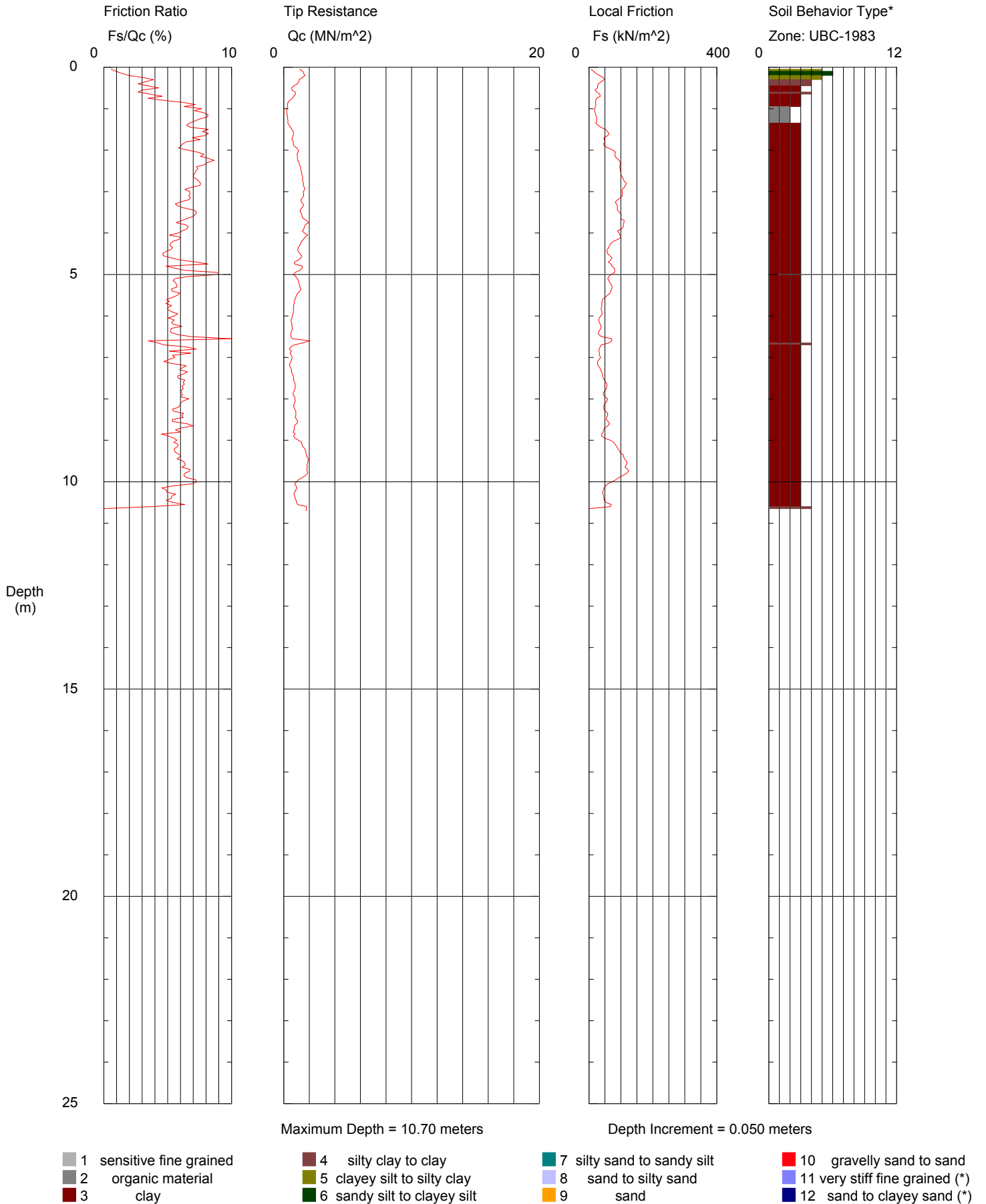
Figure 13. Hogentogler log for SNC012.
