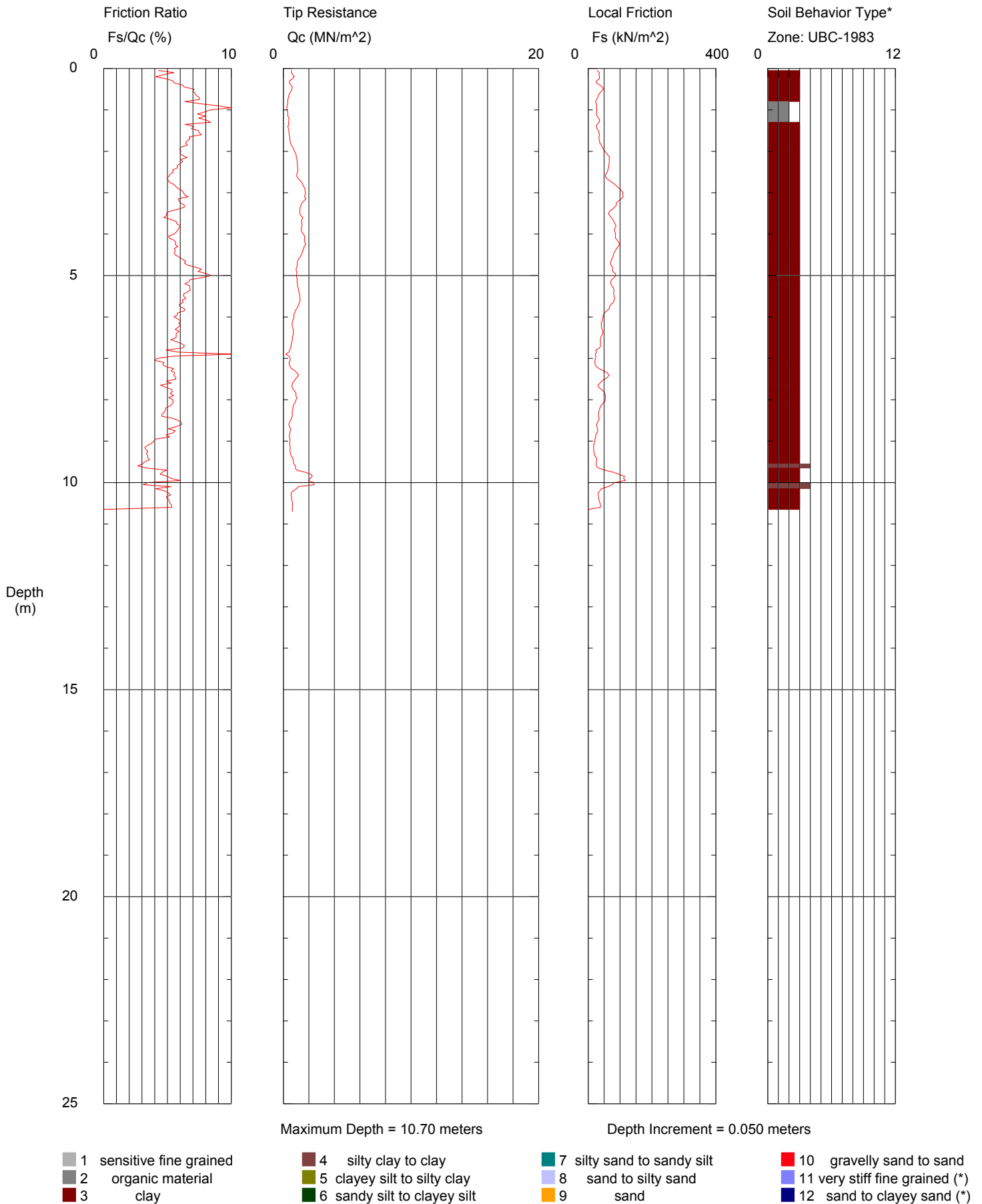
Figure 10. Hogentogler log for SNC009.
