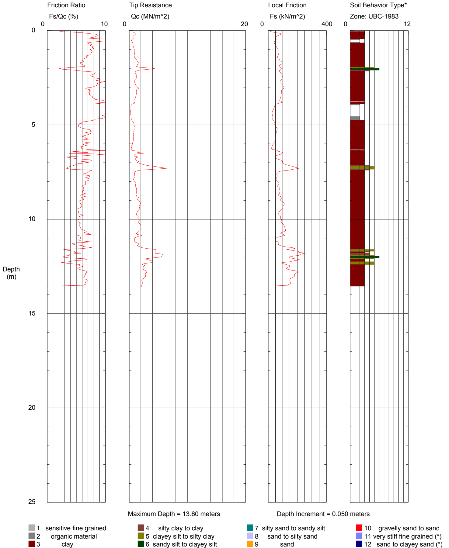
Figure 9. Hogentogler log for SNC008.
