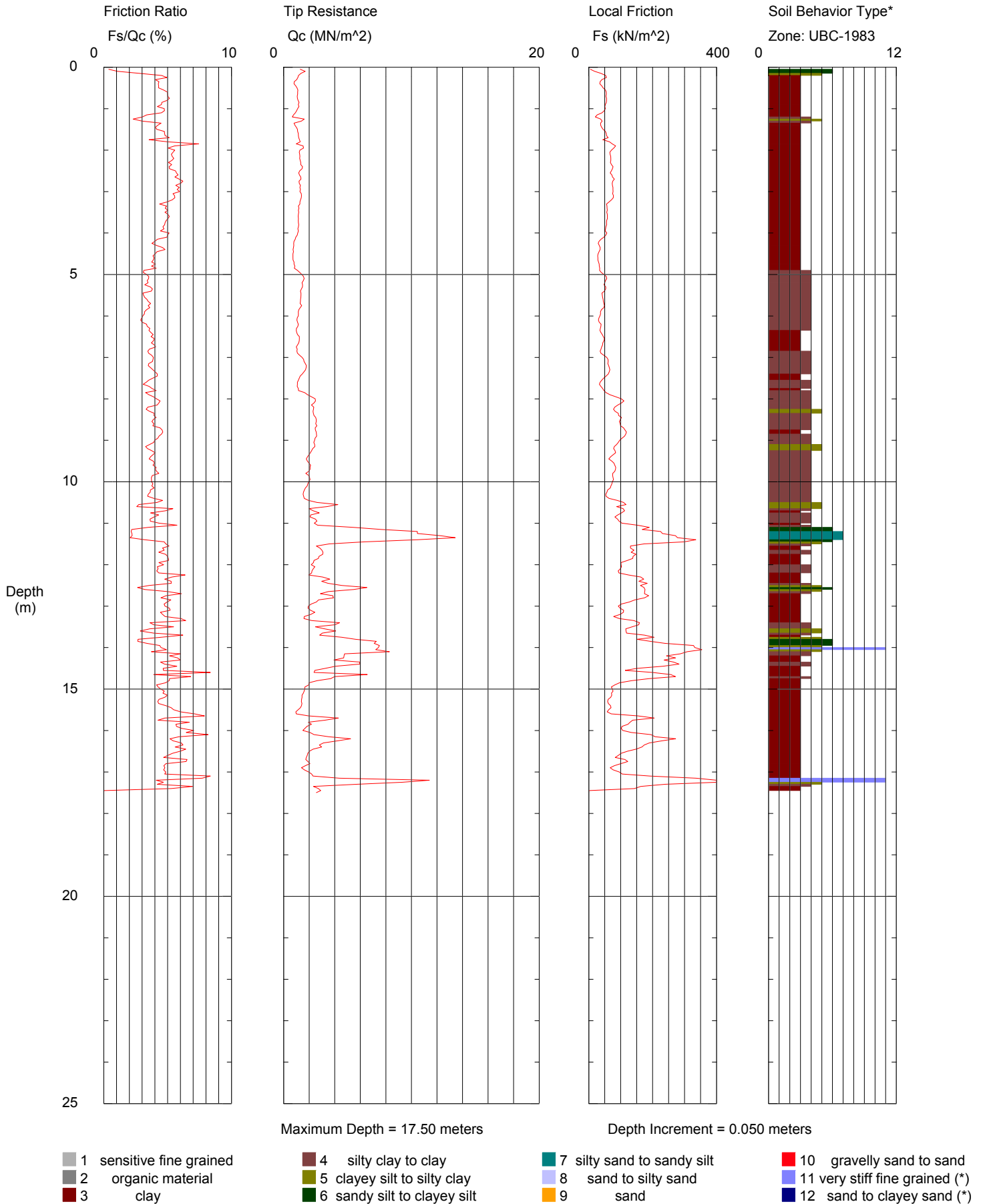
Figure 7. Hogentogler log for SNC006.
