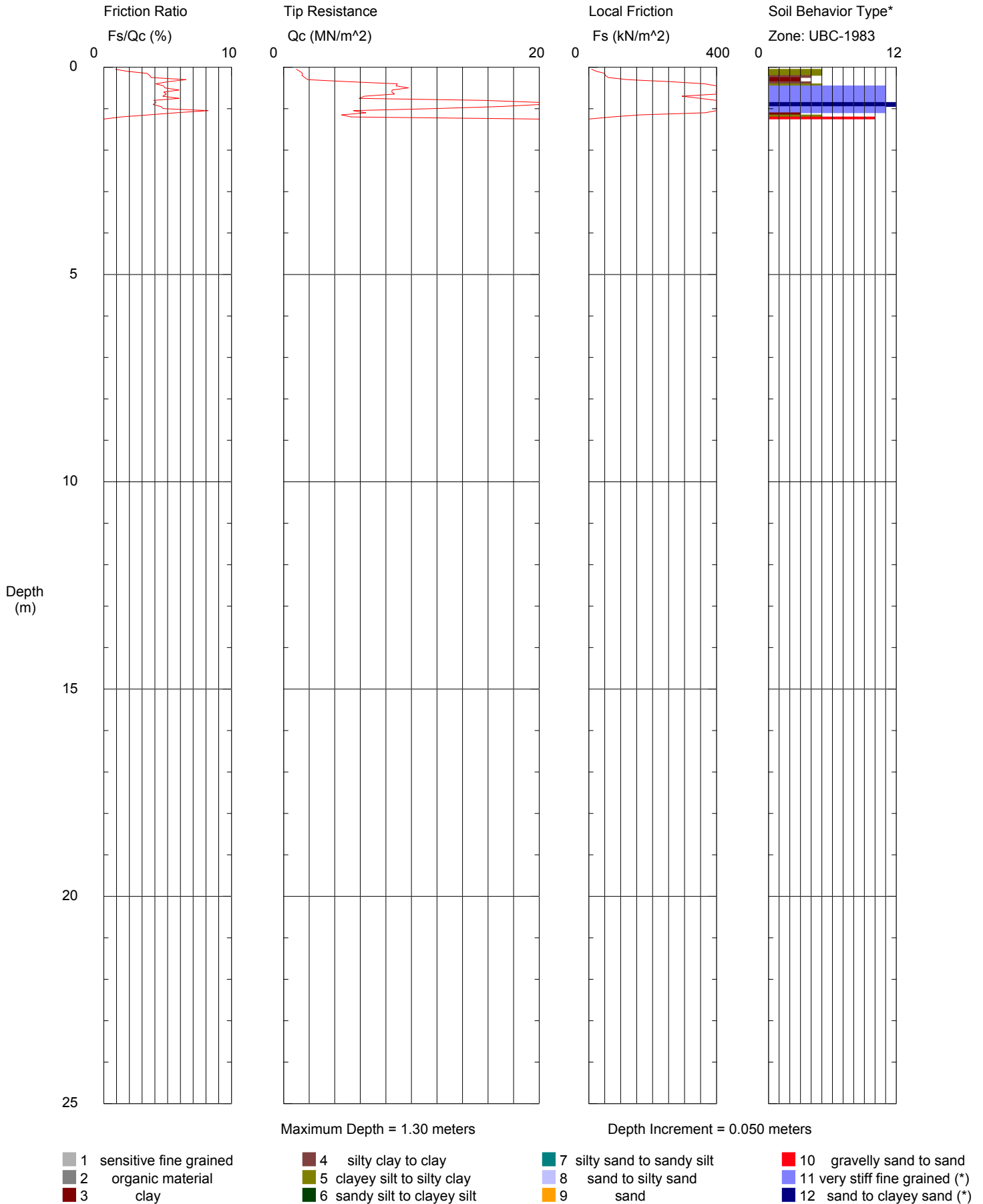
Figure 6. Hogentogler log for SNC005.
