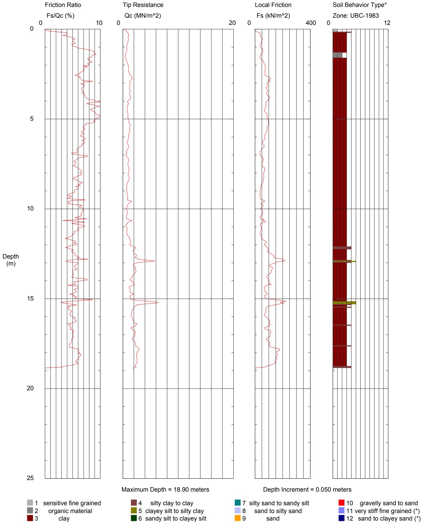
Figure 5. Hogentogler log for SNC004.
