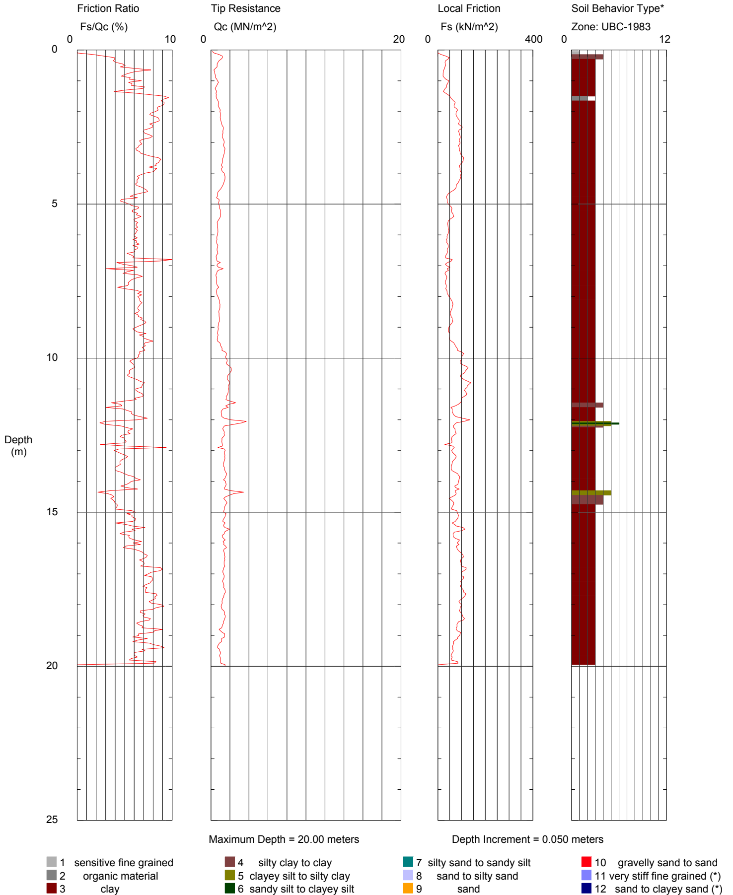
Figure 4. Hogentogler log for SNC003.
