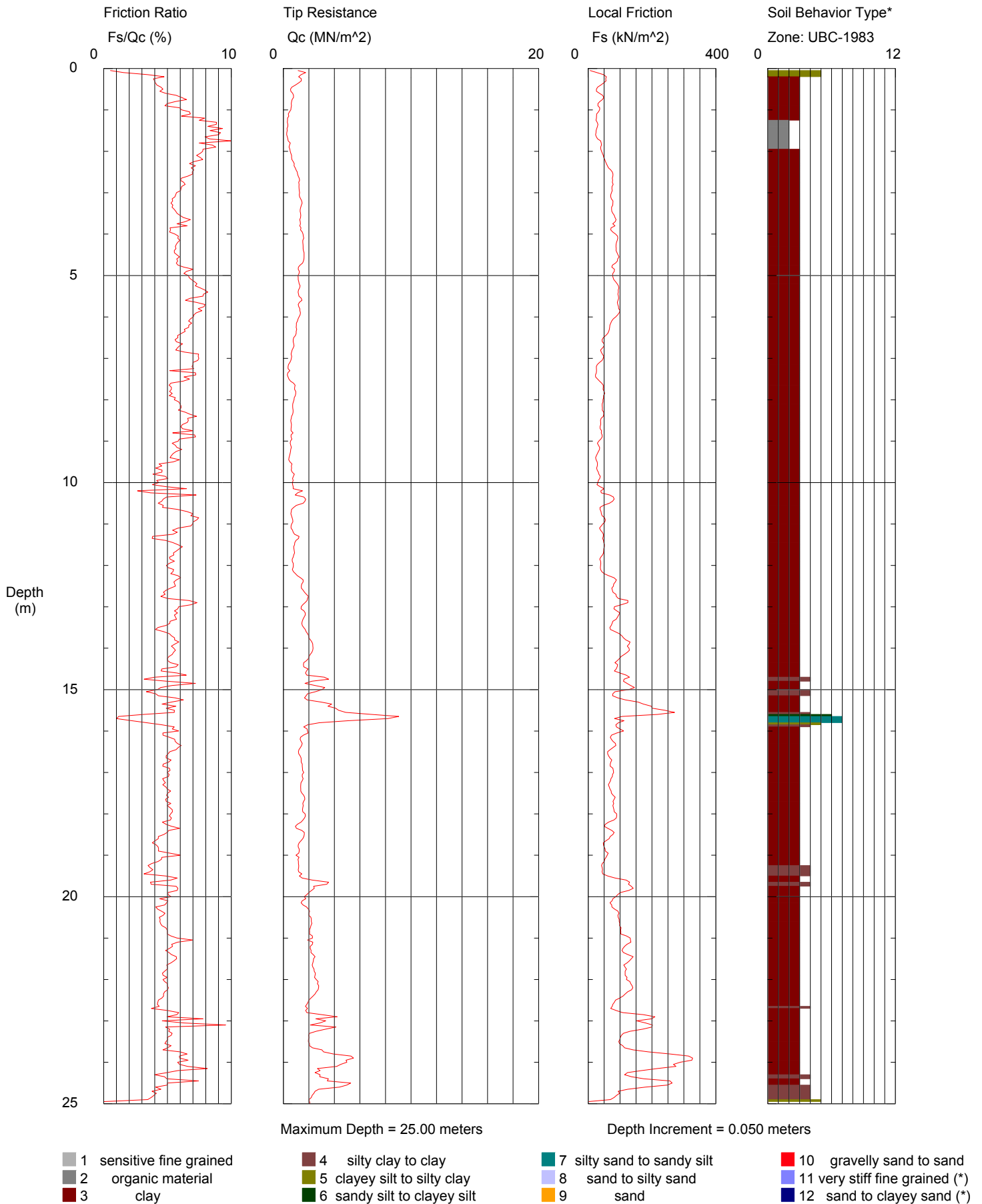
Figure 3. Hogentogler log for SNC002.
