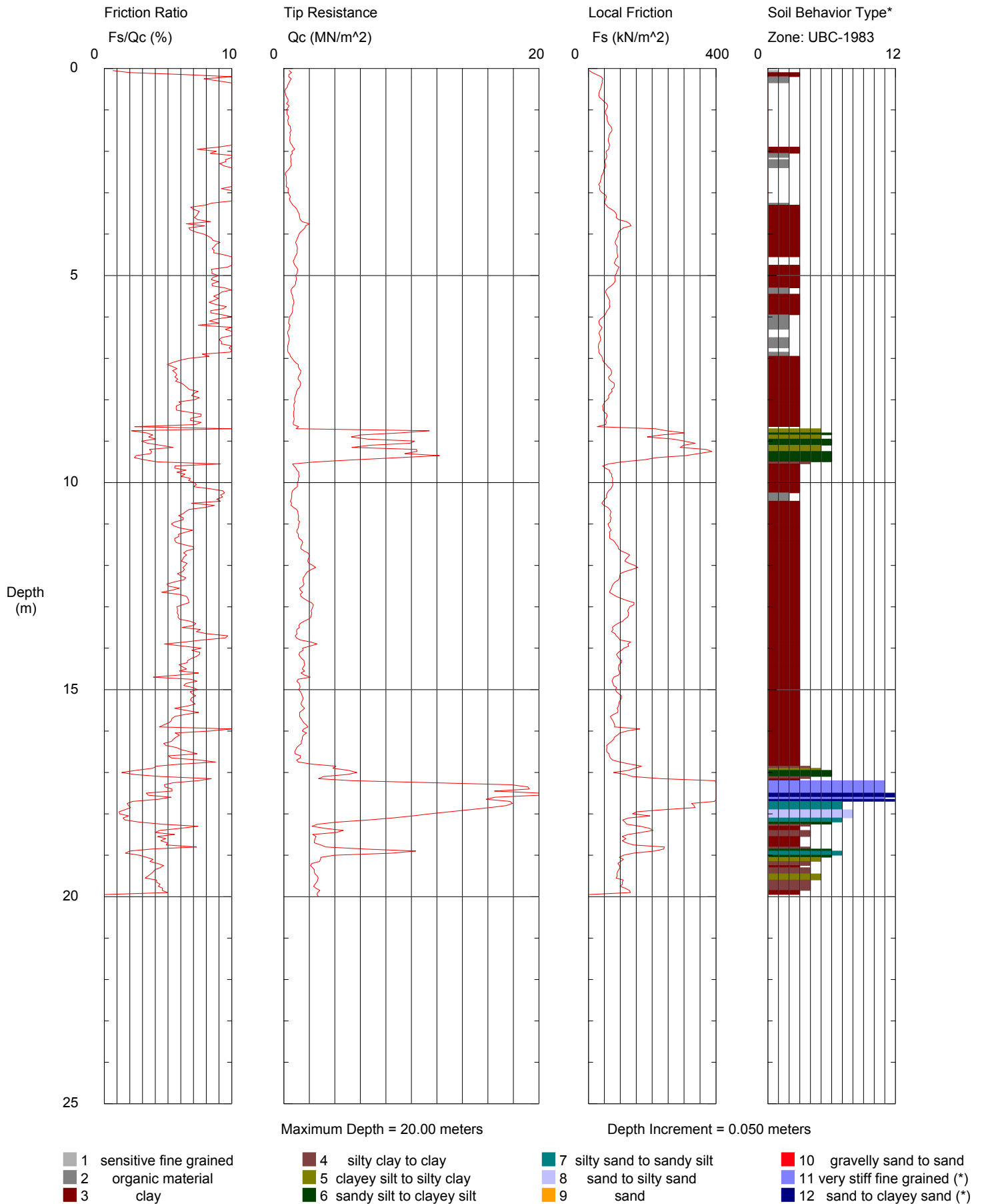
Figure 2. Hogentogler log for SNC001.
