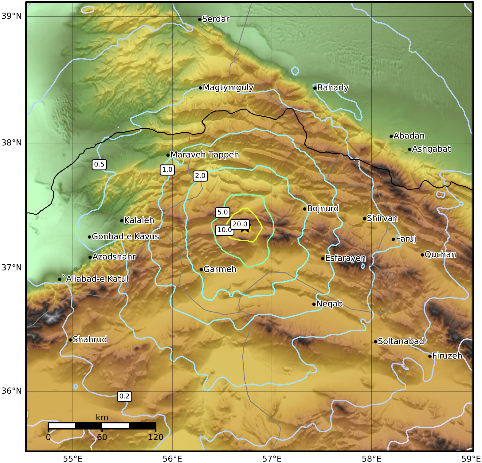
Peak Ground Acceleration Map USGS ShakeMap: 55 km WSW of Bojnūrd, North Khorasan, IR May 17, 2021 00:54:01 UTC M5.4 N37.33 E56.73 Depth: 10.0km ID:us7000e3n6
