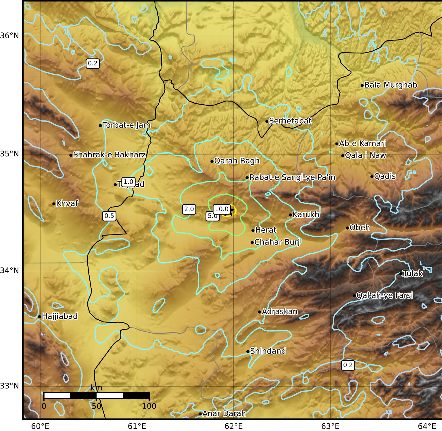
1.0 Second Peak Spectral Acceleration Map USGS ShakeMap: 26 km NE of Zindah Jān, Herat, AF Oct 07, 2023 06:49:41 UTC M5.4 N34.52 E61.95 Depth: 10.3km ID:us6000ldph
