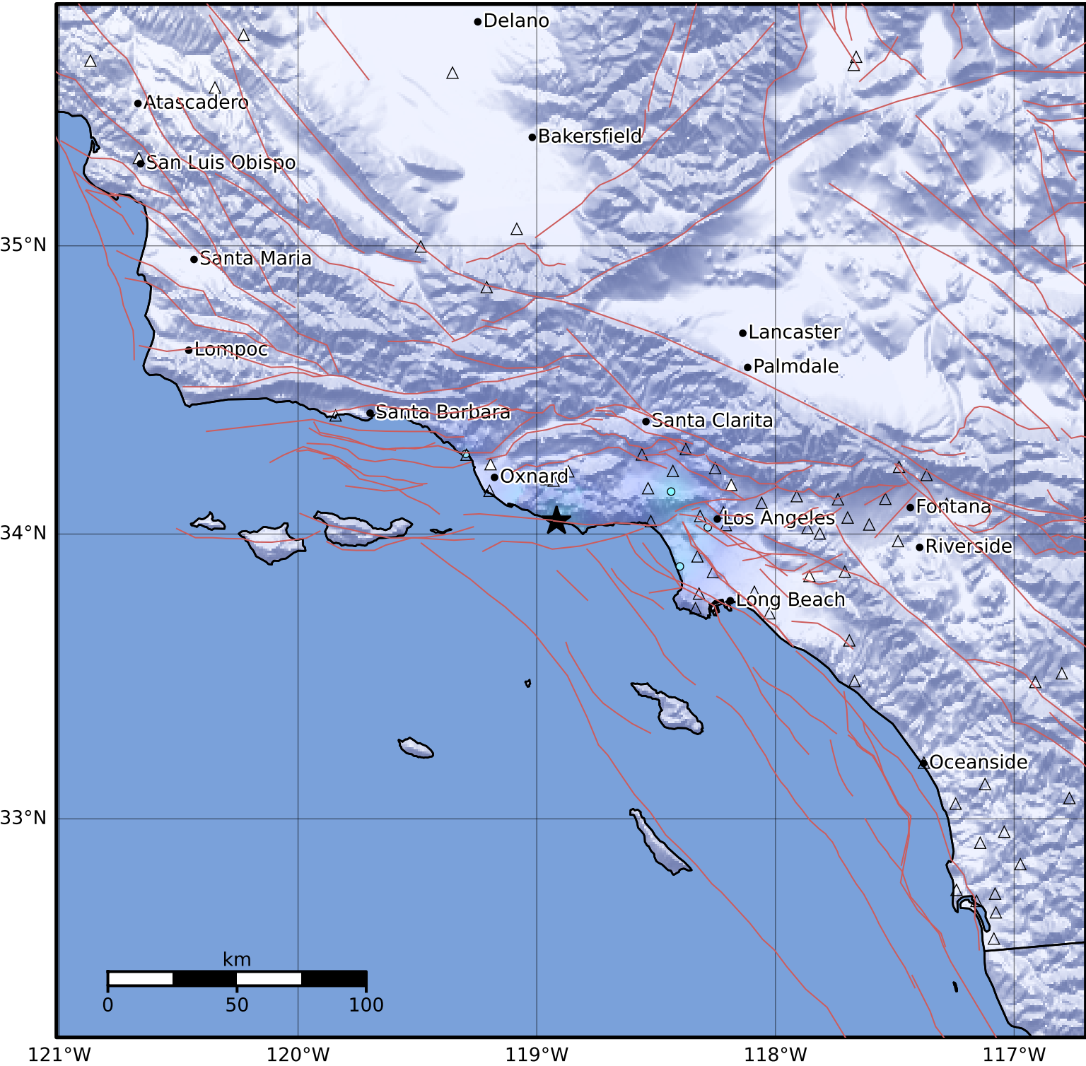
Macroseismic Intensity Map CISN/sc ShakeMap: 10.8 km (6.7 mi) WNW of Malibu, CA Feb 09, 2024 21:50:18 UTC M3.0 N34.05 W118.92 Depth: 15.0km ID:40664648
