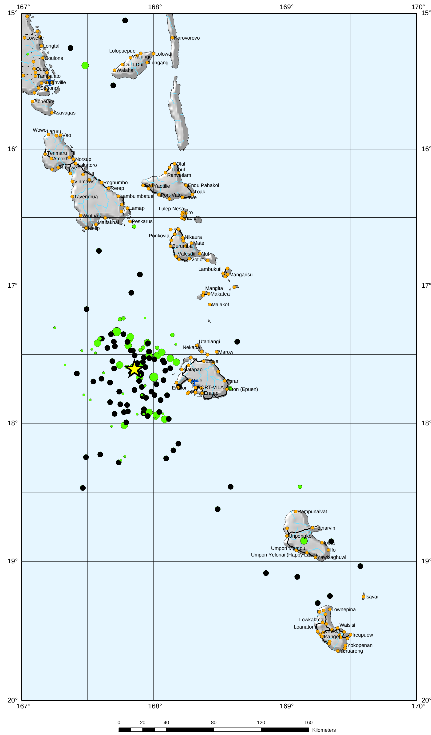
Epicentral Area
