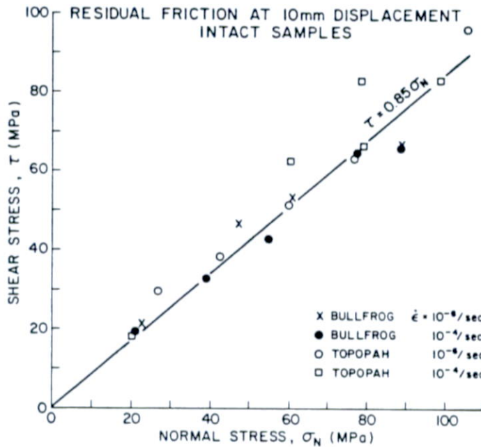
Fig. 7. Shear and normal stress data (assuming a 30^\circ fracture angle) for intact samples after 10 mm of axial displacement.
