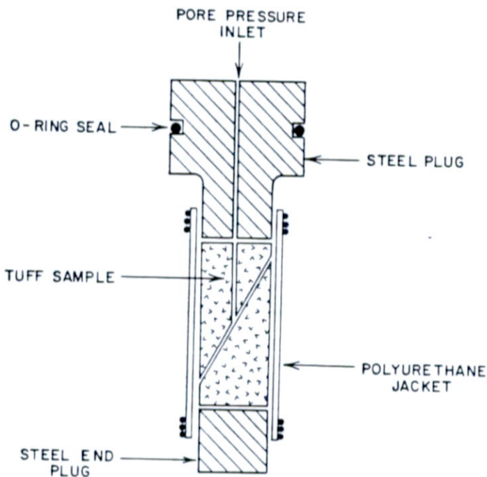
Fig. 1. Sample assembly.
