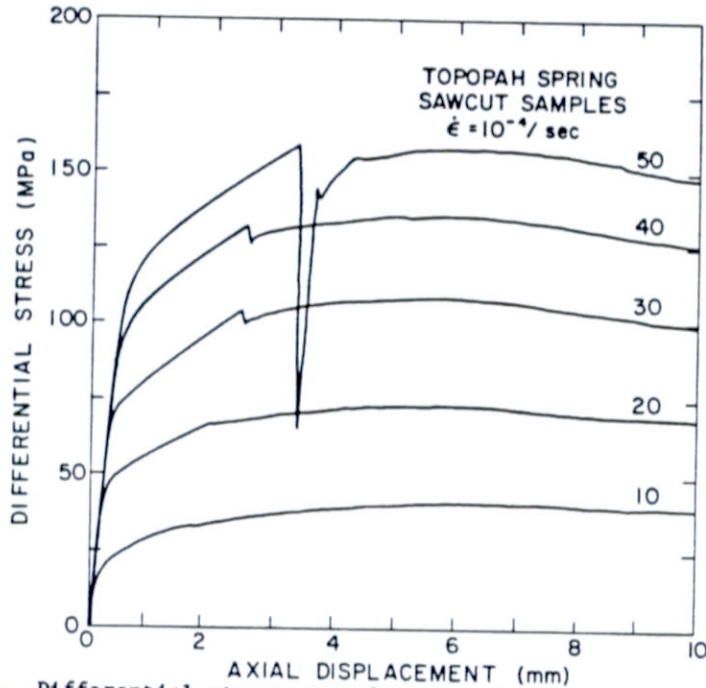
Fig. 2. Differential stress as a function of axial displacement for sawcut samples of the Topopah Spring Member at a strain rate of 10^{-4}/\text{s} . Confining pressures in MPa are shown at the right of each curve.
