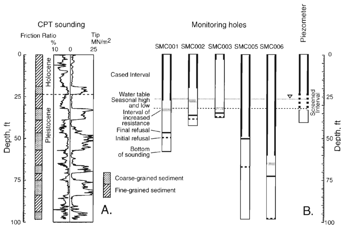
Figure 1. (a) CPT sounding profile with inferred lithology, and (b) monitoring holes and piezometer. Depths of initial and final refusal, respectively, were measured immediately and approximately three years after each sounding was completed.
